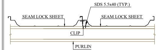
PURLIN WITH SEAM LOCK CLIP DETAIL
