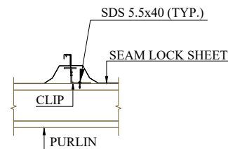
CLIP DETAIL
