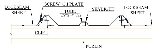
SKYLIGHT & LOCKSEAM SHEET DETAIL TYPICAL
