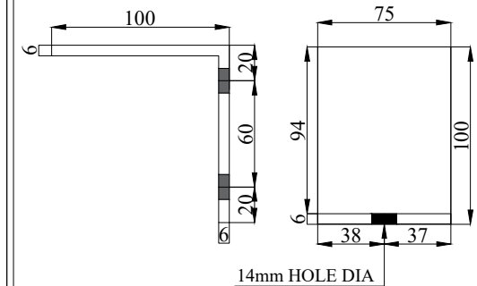
DETAIL OF [L-CLIP-100*100*75*6]
